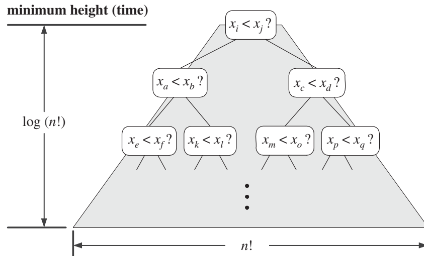
Figure 8.12: Visualizing the lower bound for comparison-based sorting.
