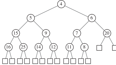
Figure 5.6: Example of a heap storing 13 integer keys. The last node is the one storing key 8, and external nodes are empty.
